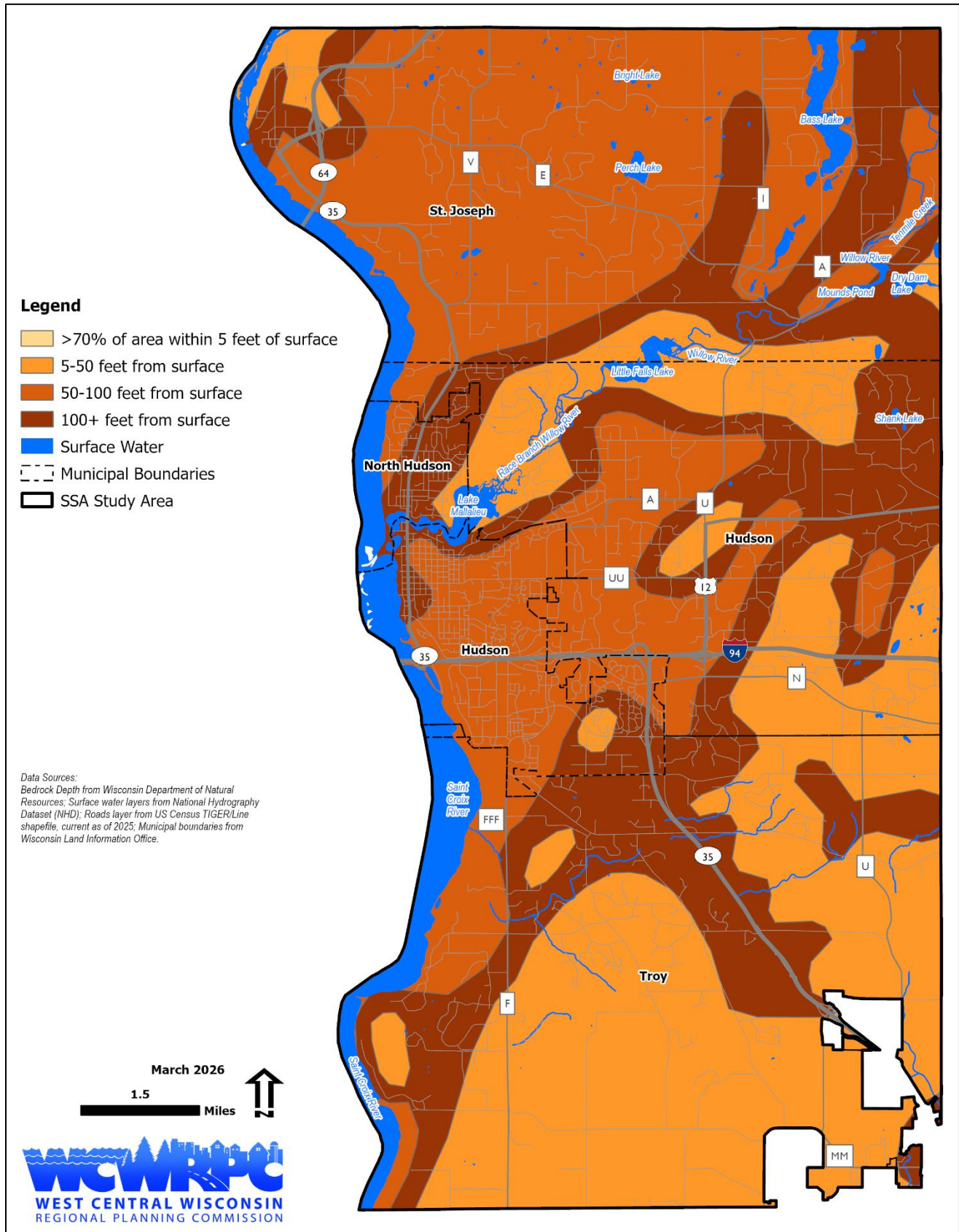
Map 3.1. Depth to Bedrock
