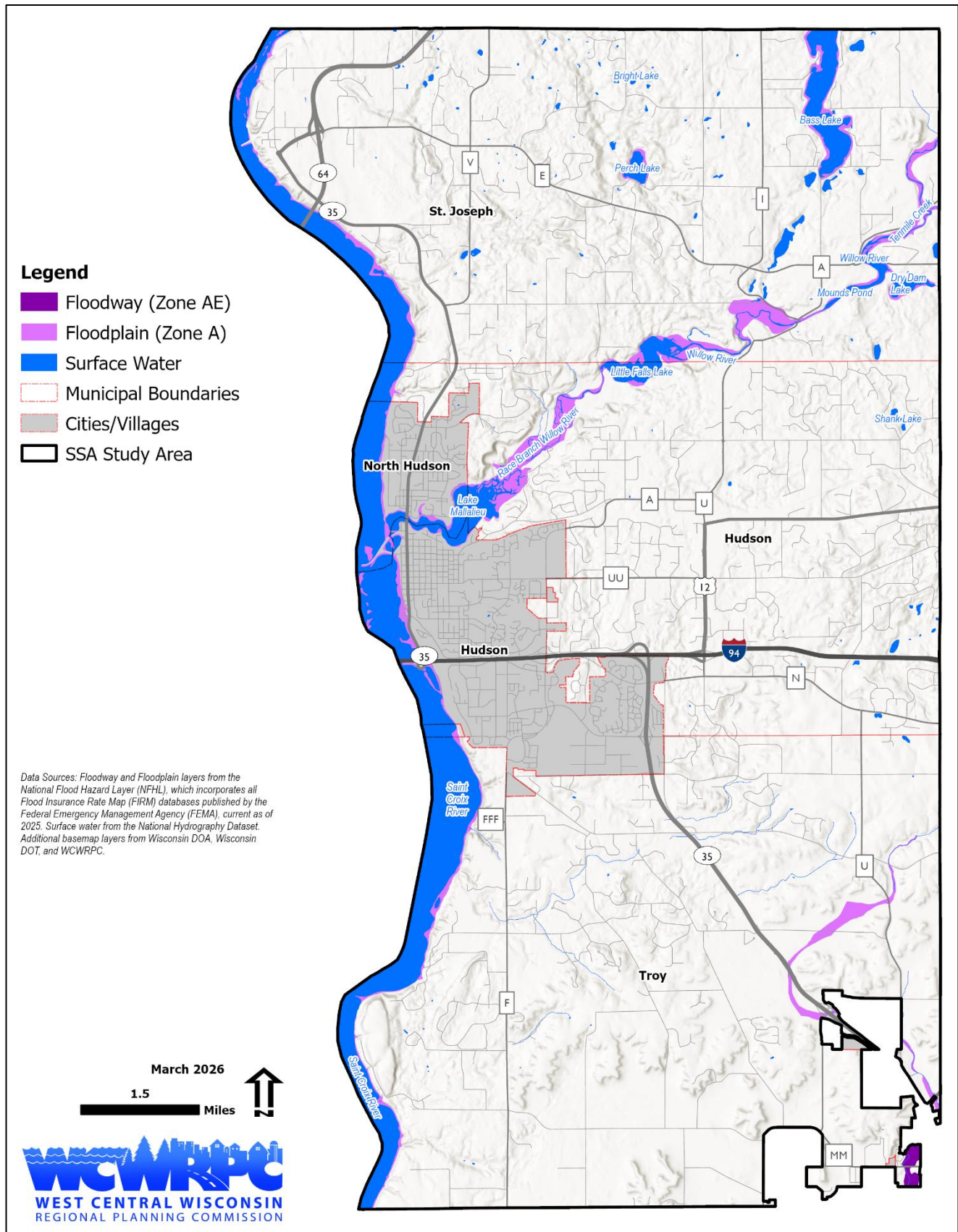
MAP 3.13 Surface Waters & 100-Year Floodplains
