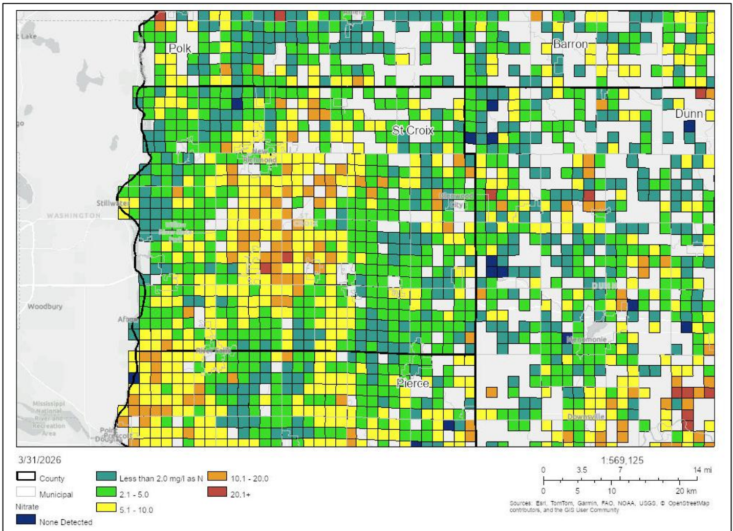
Map 3.7 Well Testing Averages for Nitrates, 1985-2024
